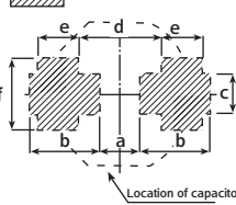
Fig.3 Resin-Molded chip type <Share with Ta/Al multilayer capacitors (7343 size) >
